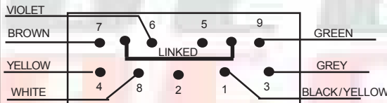
REAR VIEW OF RALLY etc. DC TYPE LIGHT SWITCH
