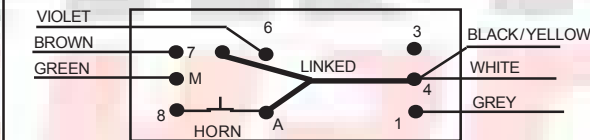
ALTERNATIVE SWITCH - REAR VIEW - V90/100/PRIM etc. AVOID THIS SWITCH - SEPERATE HORN BUTTON REQUIRED
