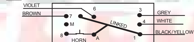
ALTERNATIVE SWITCH - REAR VIEW - ET3 / RALLY AC. AVOID THIS SWITCH - REQUIRES SEPERATE HORN BUTTON AND IGNITION CUT OUT.
