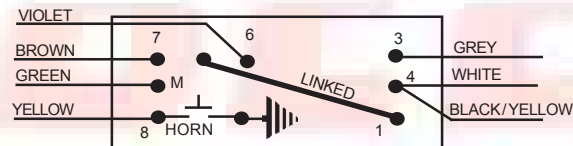
BEEDSPEED 12V CONVERSION SWITCH - REAR VIEW
